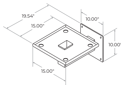
WALL MOUNT ARM DIMENSIONS
